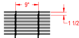
HL-9 Curtain 3/16" 2-Hole Links Links 9" OC - Rods 1 1/2" OC
