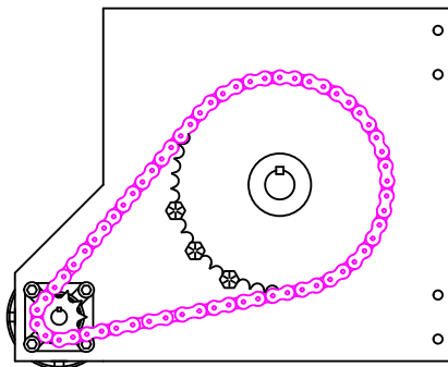
Compound Tension Bracket
