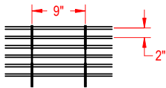
SL-9 Curtain Single 1/8" & Double 1/16" 3-Hole Links Links 9" OC - Rods 2" OC
