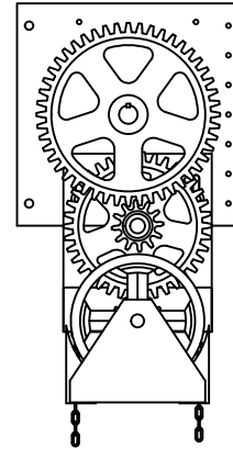
Multiple Gear Reduction
