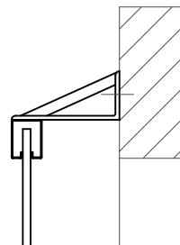
OPTIONAL EXTENDED TOP BRACKET
