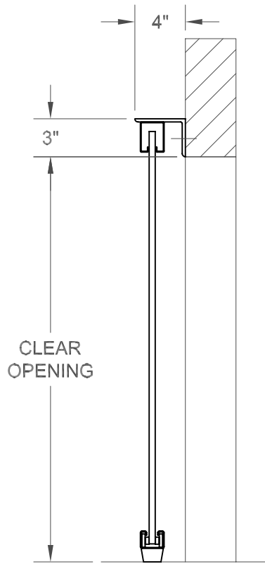
FACE MOUNT INVERTED TOP BRACKET
