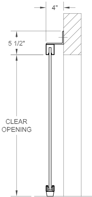
FACE MOUNT STANDARD TOP BRACKET
