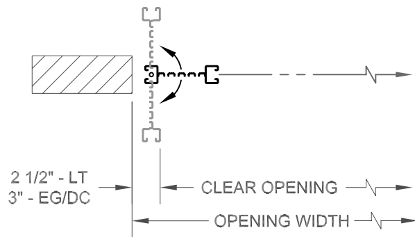
BETWEEN JAMB MOUNT
