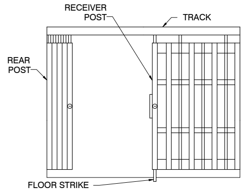
BI-PARTING
