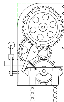
CHAIN BRACKET (MOTOR SIMILAR)
