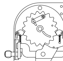
PUSH-UP BRACKET (CHAIN SIMILAR)
