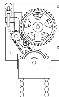
CHAIN BRACKET (MOTOR SIMILAR)
