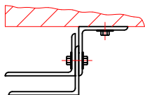
3pc. Angle Guide (Doors Over 24' Wide, Z-Guide Shown, Other Types Similar)
