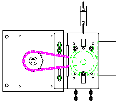
Bent Mounting Plate
