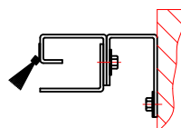
Between Jamb Mount (Shown With Brush Seal)
