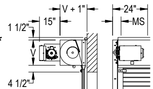
MOTOR OPERATOR* MODEL: HWFM
